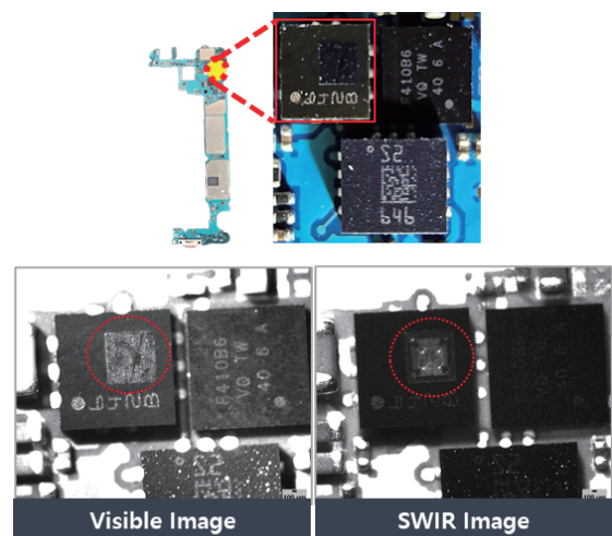
* Sample : Samsung Galaxy A7(2017) PCB
