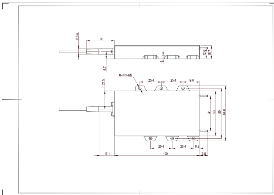
尺寸外观 (Dimension appearance)
