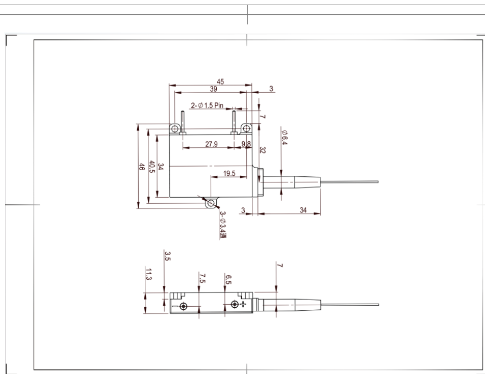
■ 尺寸外观 (Dimension appearance)
